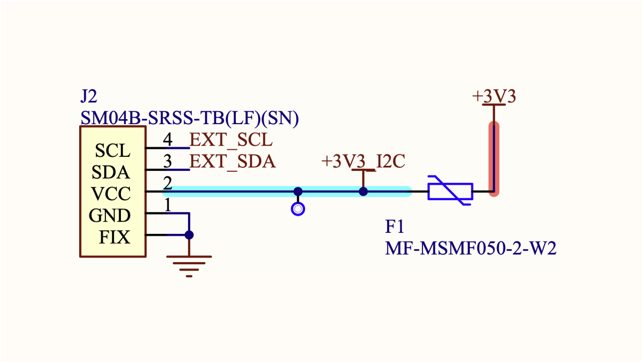
I2C .
